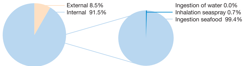
Figure 3.18: Contribution of exposure pathway to the committed effective dose for high seafood consumers as a function of age group (K4 ALPS treated water tank group)
